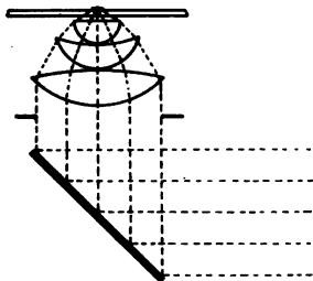
Fig. 52. Illuminating object with condenser and plane mirror. The right way.
